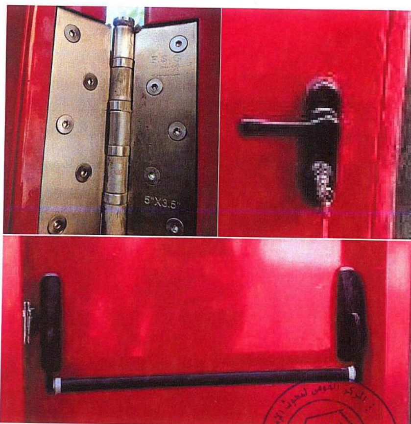
Figure (2): Hardware and accessories of the test door assembly.
